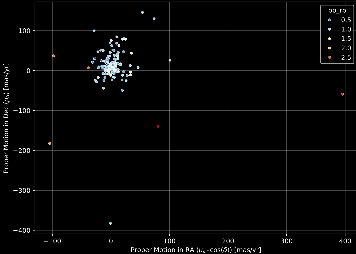
APOGEE DR17 Field: [284-30-O_TESS] Proper Motion Diagram (n= 169)
