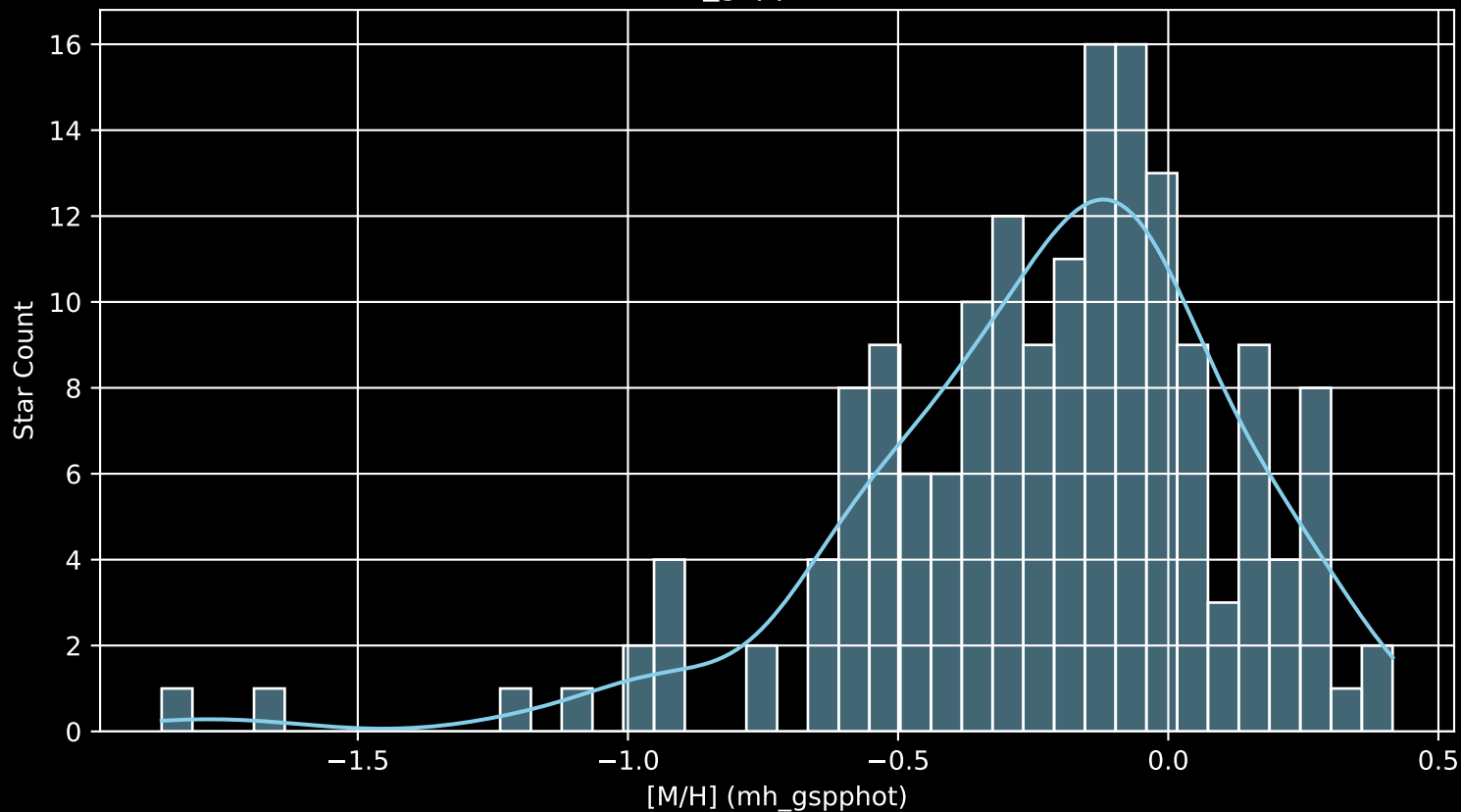
APOGEE DR17 Field: [284-30-O_TESS [M/H] (mh_gspphot) (n= 168)
