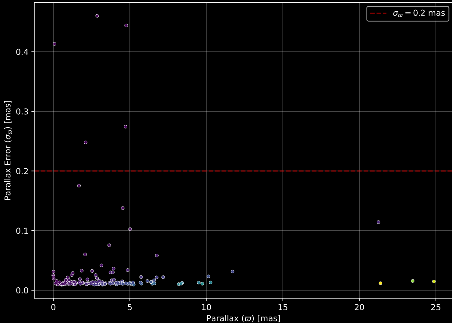
APOGEE DR17 Field: [284-30-O_TESS] Parallax Quality (n= 169)
