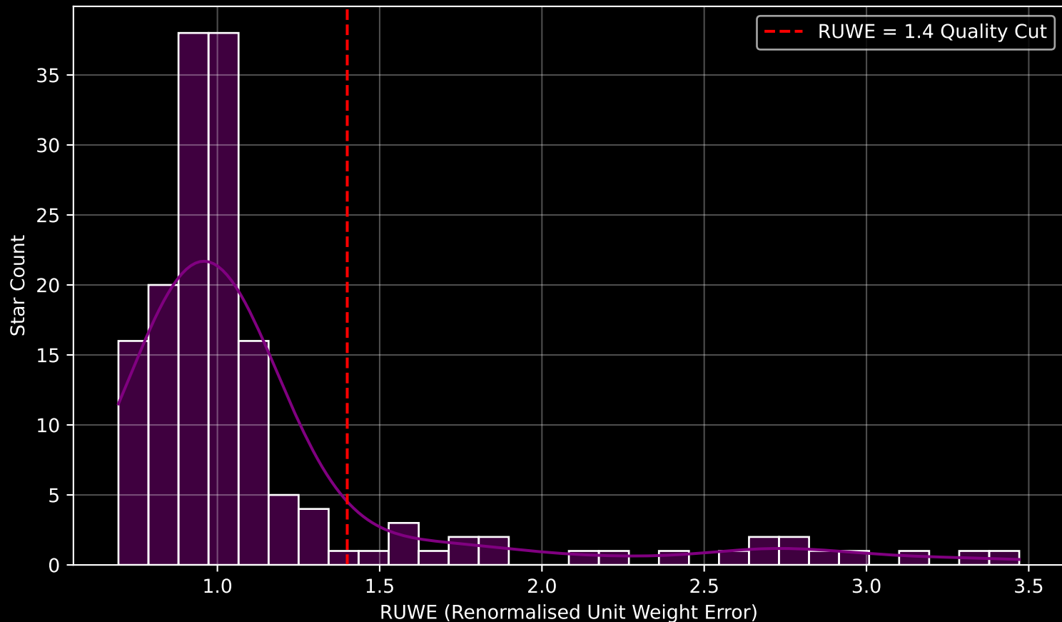
GAPOGEE DR17 Field [284-30-O_TESS] RUWE Distribution (n= 160)
