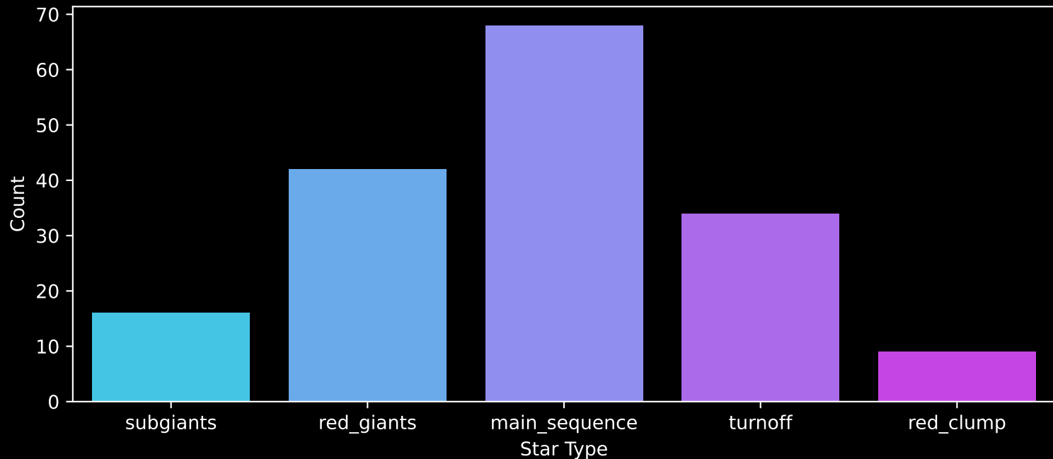
APOGEE DR17 Field: [284-30-O_TESS] Count plot of Star Type
